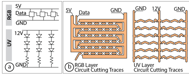
Figure 7: PortaChrome LED Layout: (a) schematics of LEDs; (b) laser-cut copper mesh for the 6x6 pixel RGB and UV circuits in the PortaChrome light source.
