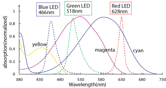
Figure 5: LED wavelength spectrum compared with the absorption spectrum of the CMY color channels.
