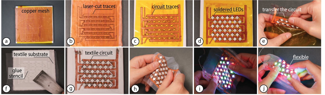
Figure 4: PortaChrome Fabrication Pipeline: We fabricate the RGB and UV circuit layers by (a-c) laser cutting the conductive traces from copper mesh, (d) soldering the LEDs, and (e-g) transferring the circuit to a textile substrate to (h-j) allow for a translucent and flexible result.
